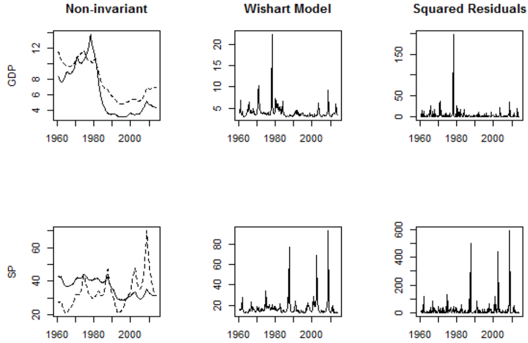
Figure 2: Estimated reduced form volatilities and squared Bayesian residuals for the real GDP growth rate (GDP) and the real stock returns (SP). The left panel corresponds to the method of Carriero et al. (2016) under two different orderings: the solid line is for ordering 1 and the dotted line is for ordering 2. The central panel corresponds to our method with r_1 = 7 , and the right panel are the squared of the Bayesian residuals.
